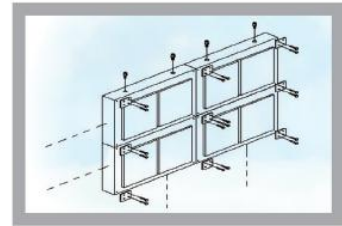
3. Assemble cabinets
